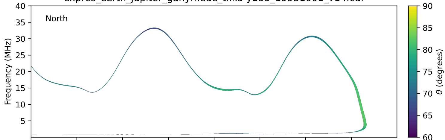
expres_earth_jupiter_ganymede_txka-y235_19931001_v14.cdf
