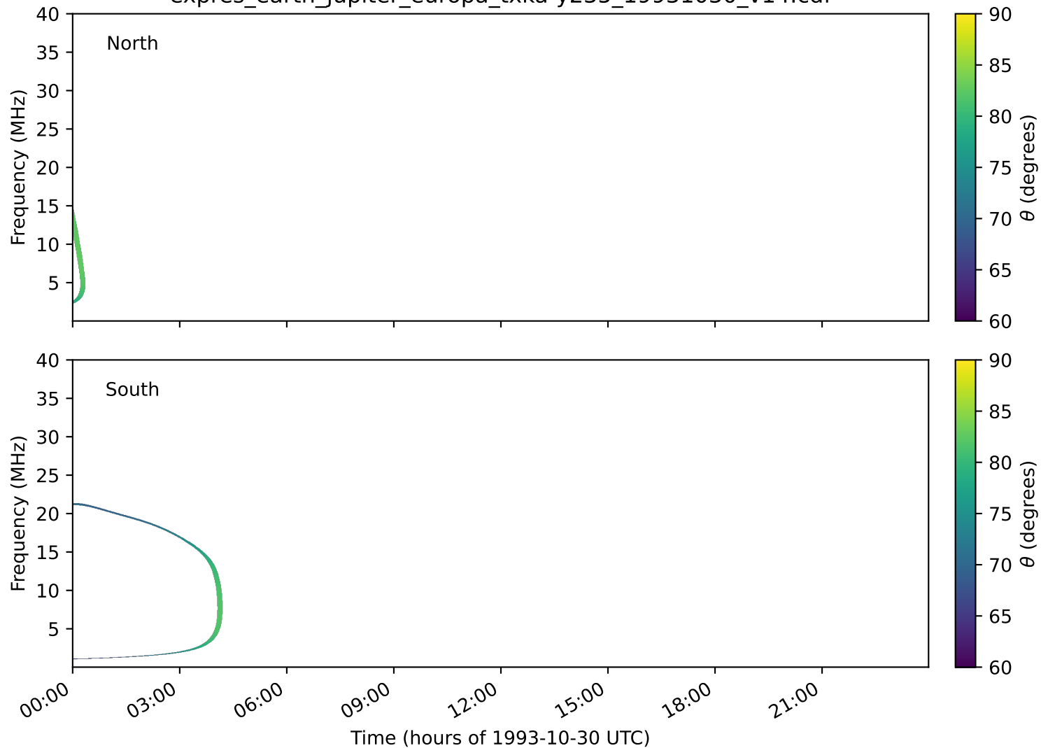
expres_earth_jupiter_europa_txka-y235_19931030_v14.cdf
