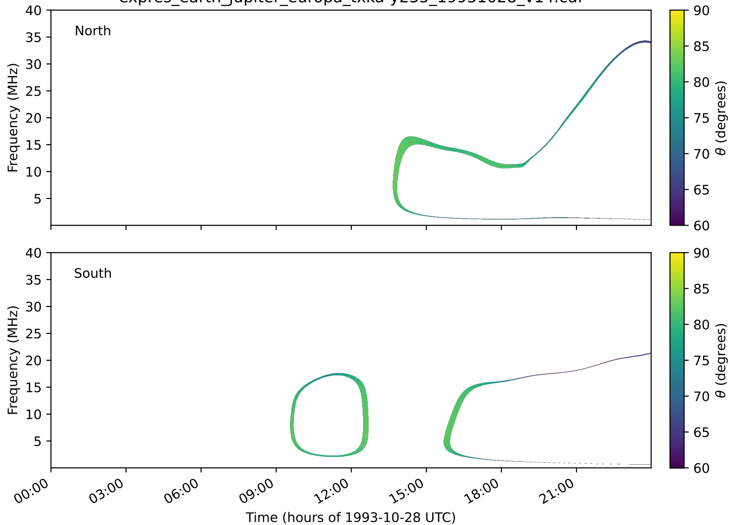
expres_earth_jupiter_europa_txka-y235_19931028_v14.cdf
