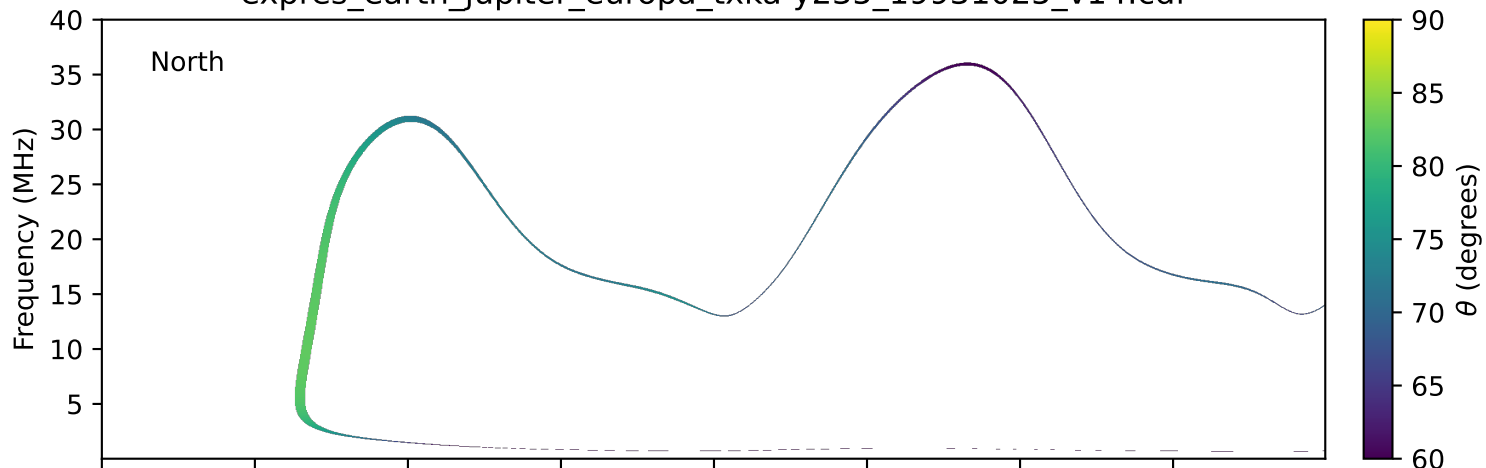
expres_earth_jupiter_europa_txka-y235_19931025_v14.cdf
