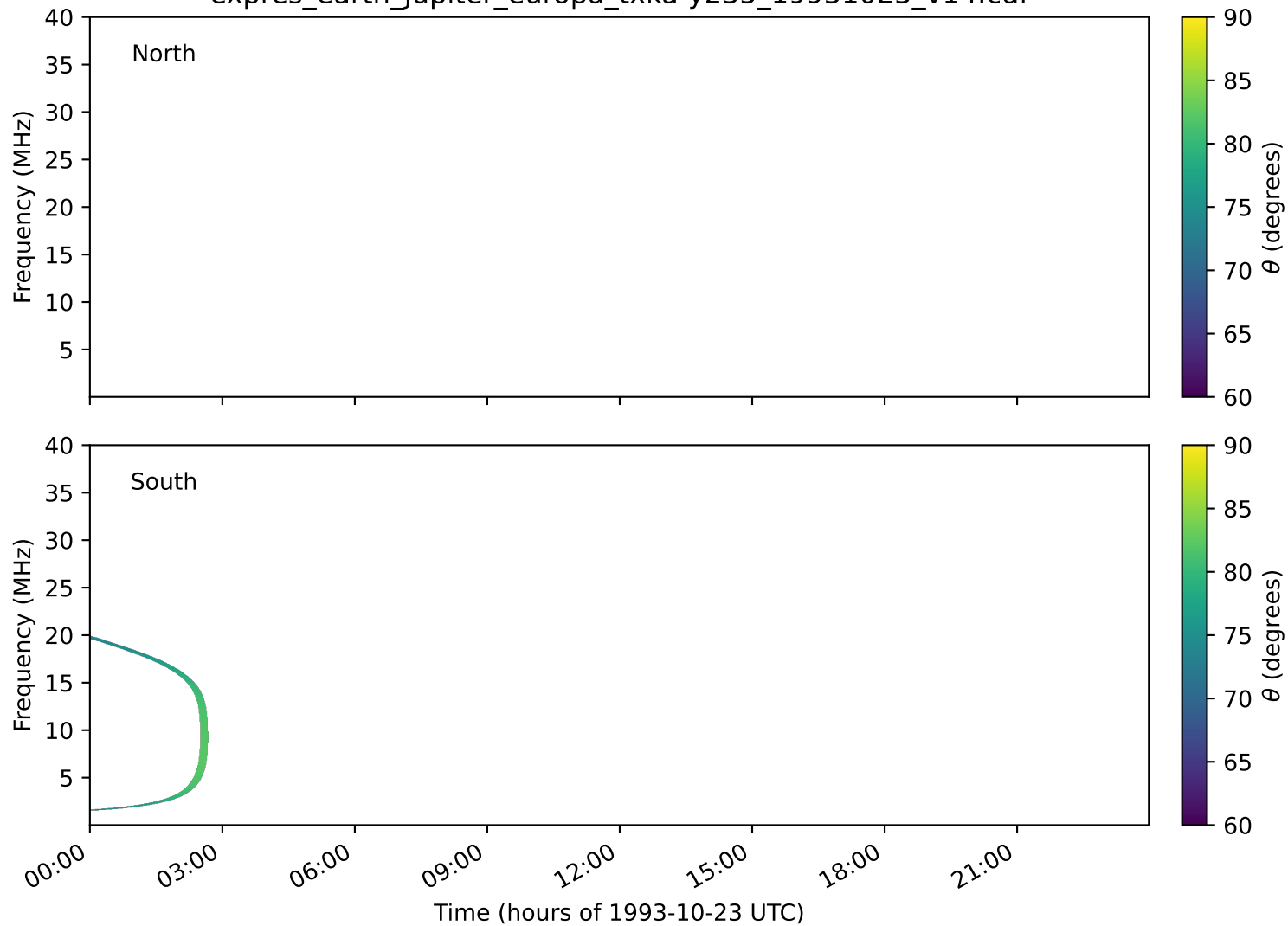
expres_earth_jupiter_europa_txka-y235_19931023_v14.cdf
