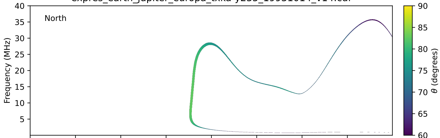
expres_earth_jupiter_europa_txka-y235_19931014_v14.cdf
