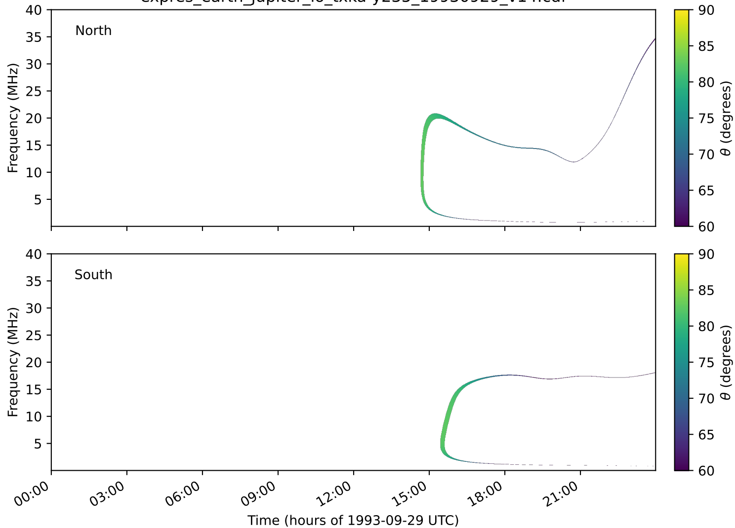
expres_earth_jupiter_io_txka-y235_19930929_v14.cdf
