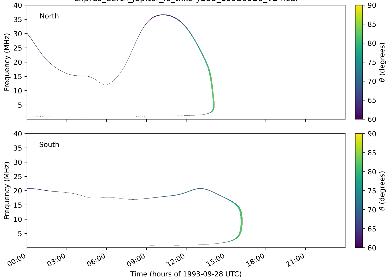
expres_earth_jupiter_io_txka-y235_19930928_v14.cdf
