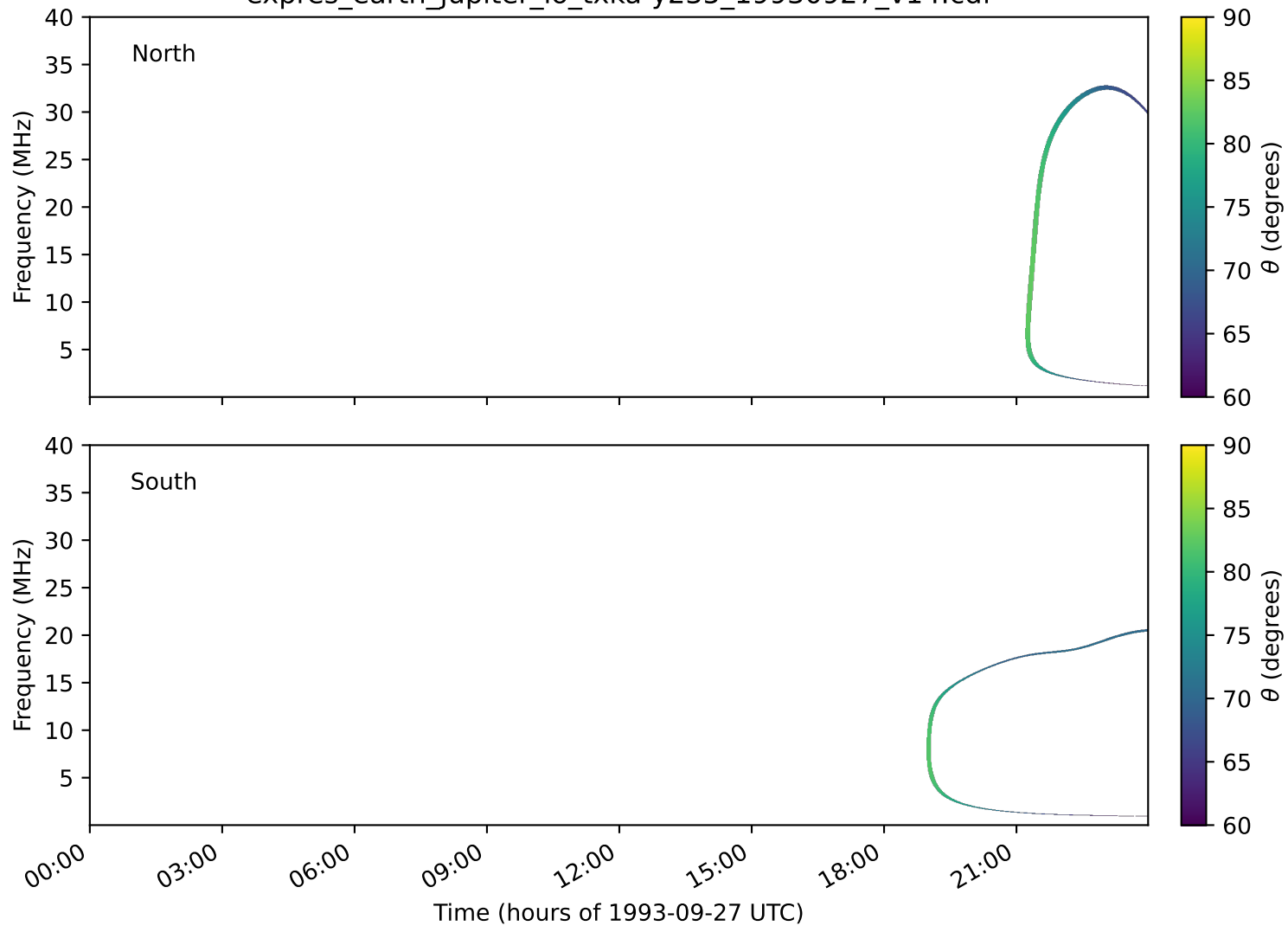
expres_earth_jupiter_io_txka-y235_19930927_v14.cdf
