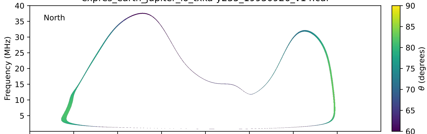
expres_earth_jupiter_io_txka-y235_19930926_v14.cdf
