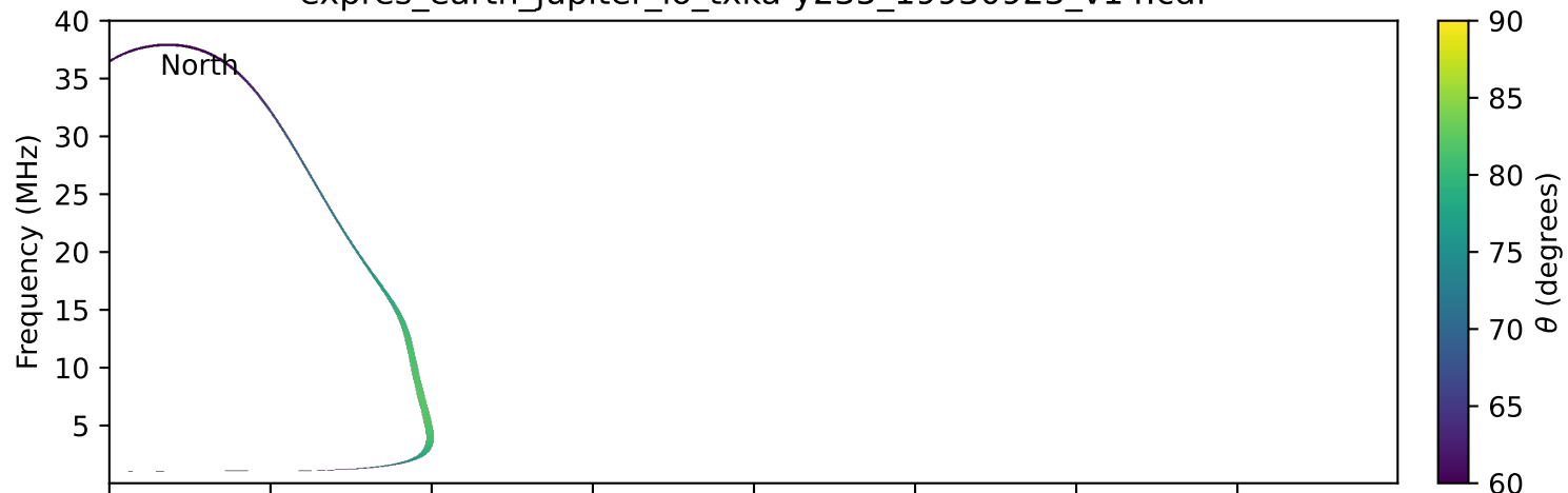
expres_earth_jupiter_io_txka-y235_19930923_v14.cdf
