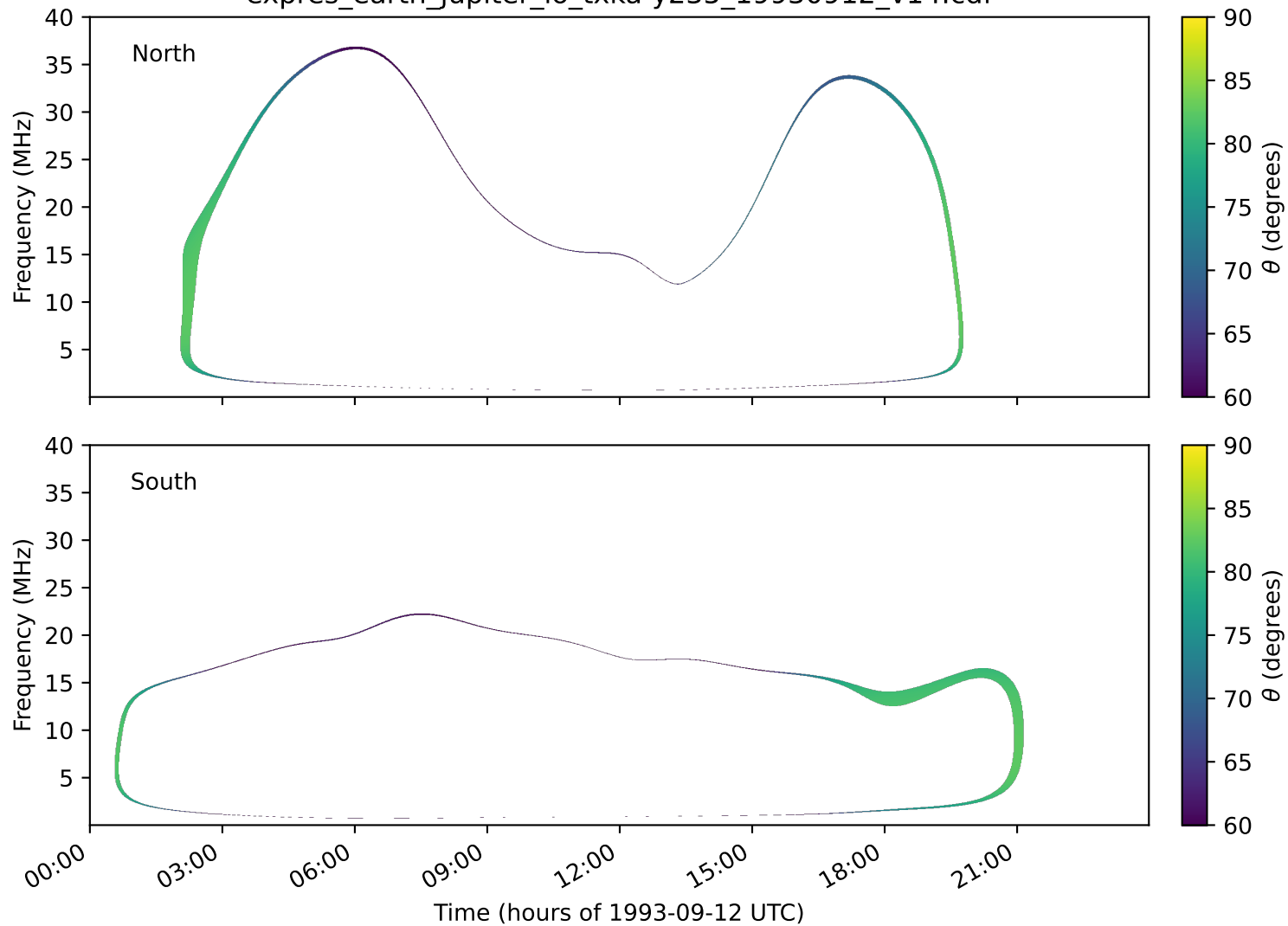
expres_earth_jupiter_io_txka-y235_19930912_v14.cdf
