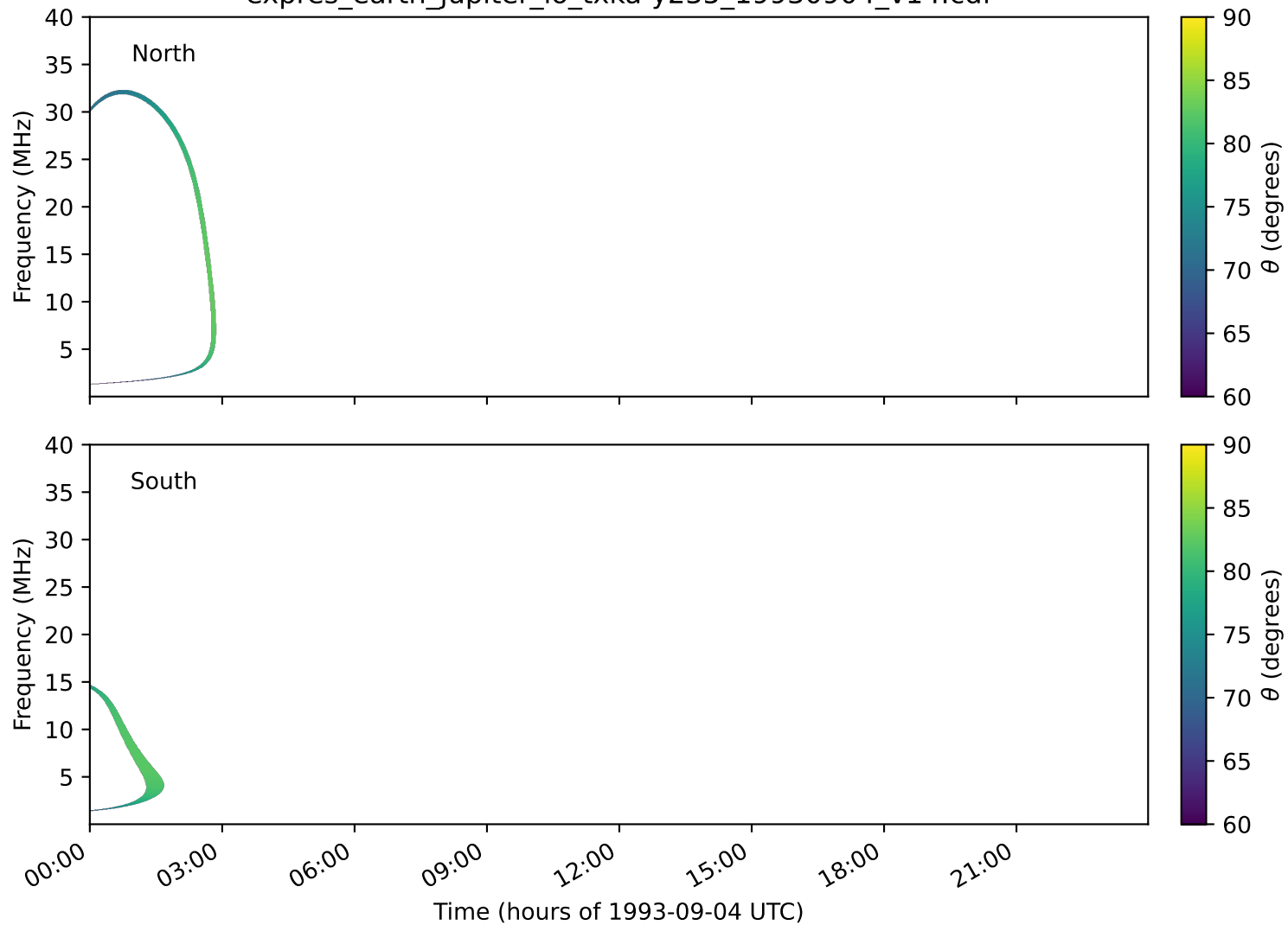
expres_earth_jupiter_io_txka-y235_19930904_v14.cdf
