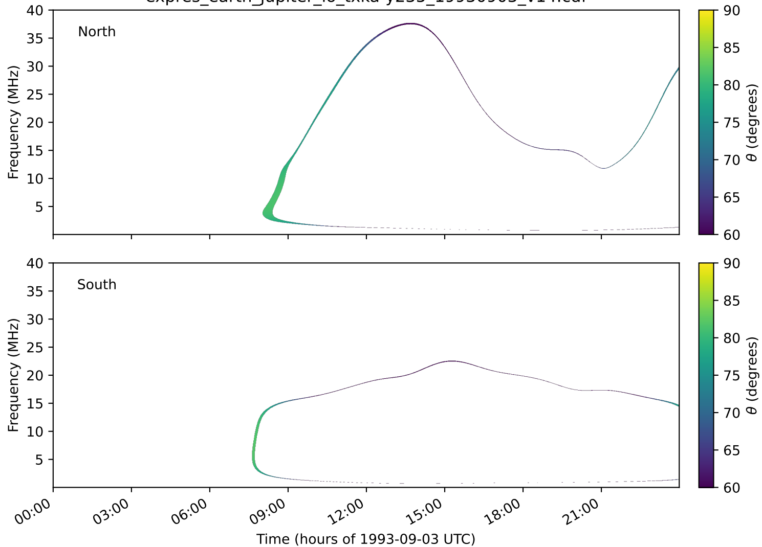
expres_earth_jupiter_io_txka-y235_19930903_v14.cdf
