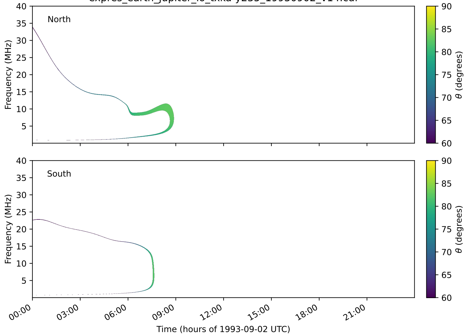
expres_earth_jupiter_io_txka-y235_19930902_v14.cdf
