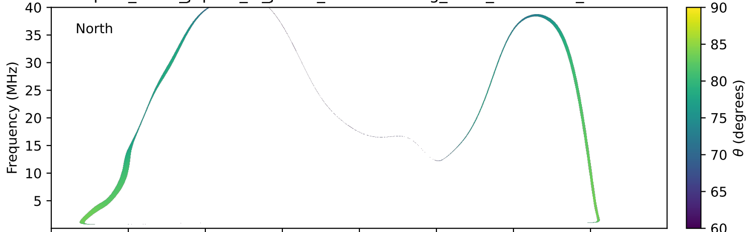
expres_earth_jupiter_io_jrm33_lossc-wid1deg_3kev_19930926_v11.cdf
