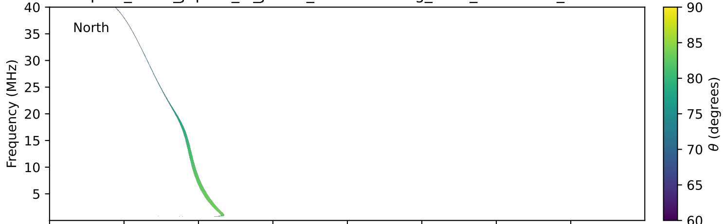
expres_earth_jupiter_io_jrm33_lossc-wid1deg_3kev_19930923_v11.cdf
