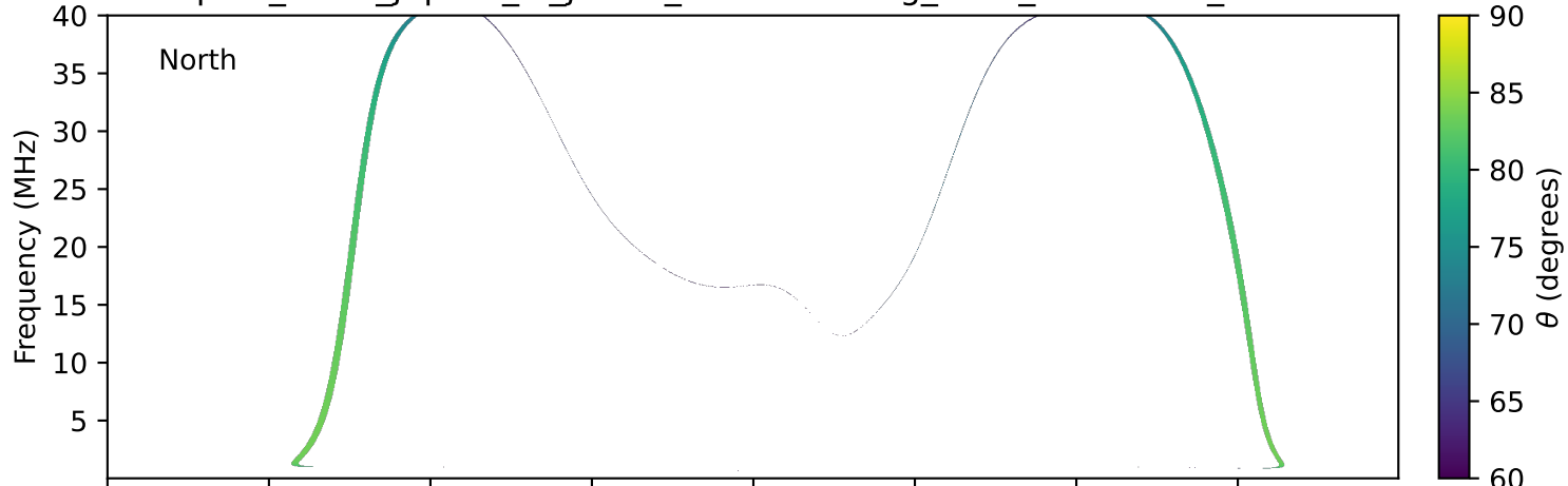
expres_earth_jupiter_io_jrm33_lossc-wid1deg_3kev_19930919_v11.cdf
