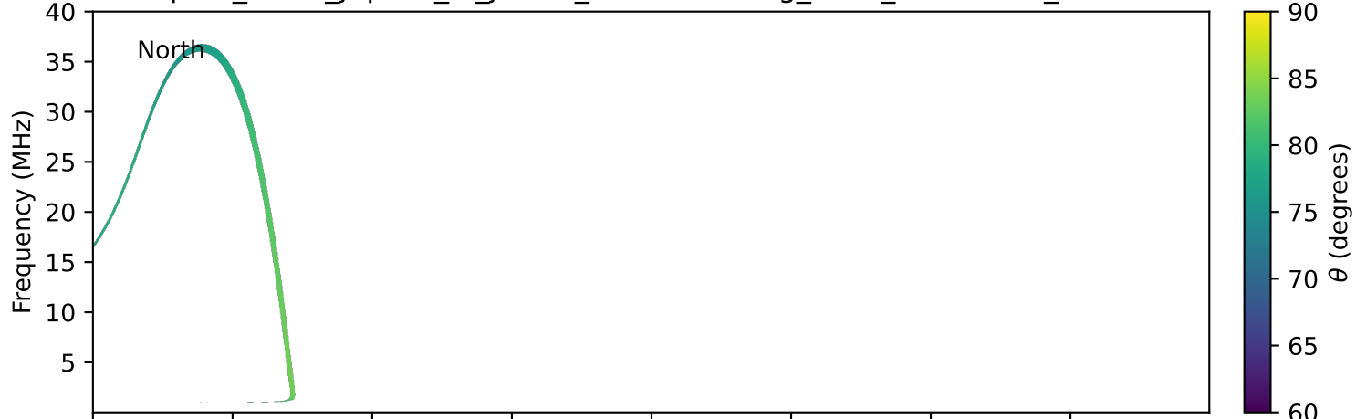
expres_earth_jupiter_io_jrm33_lossc-wid1deg_3kev_19930918_v11.cdf
