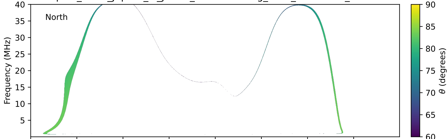
expres_earth_jupiter_io_jrm33_lossc-wid1deg_3kev_19930912_v11.cdf
