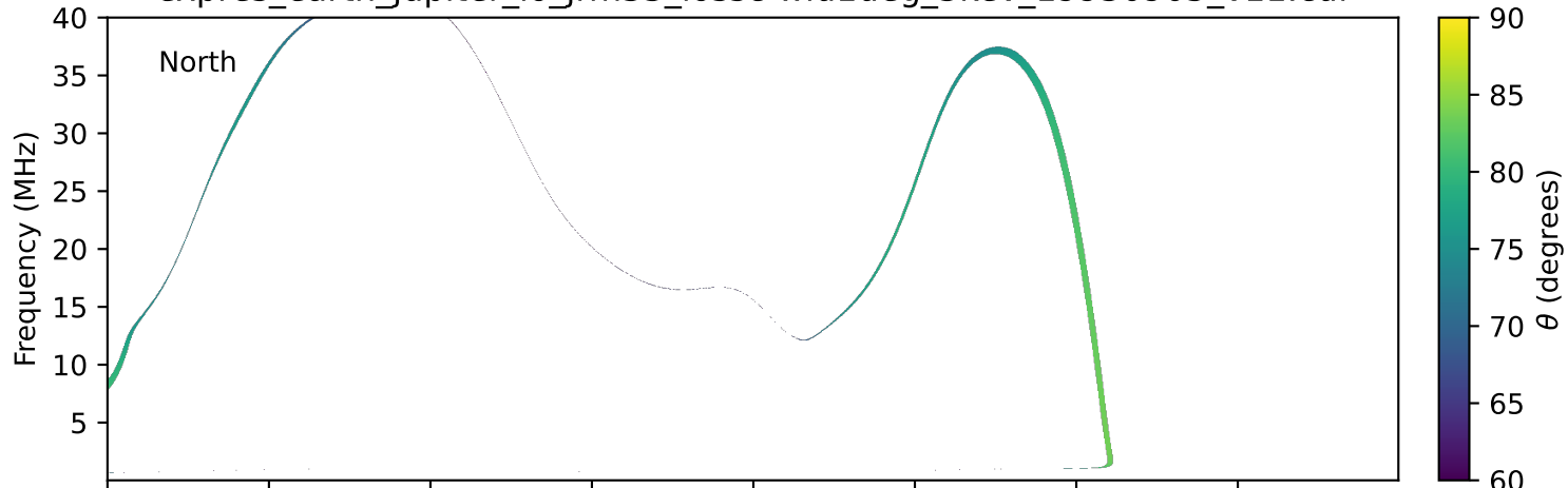
expres_earth_jupiter_io_jrm33_lossc-wid1deg_3kev_19930905_v11.cdf
