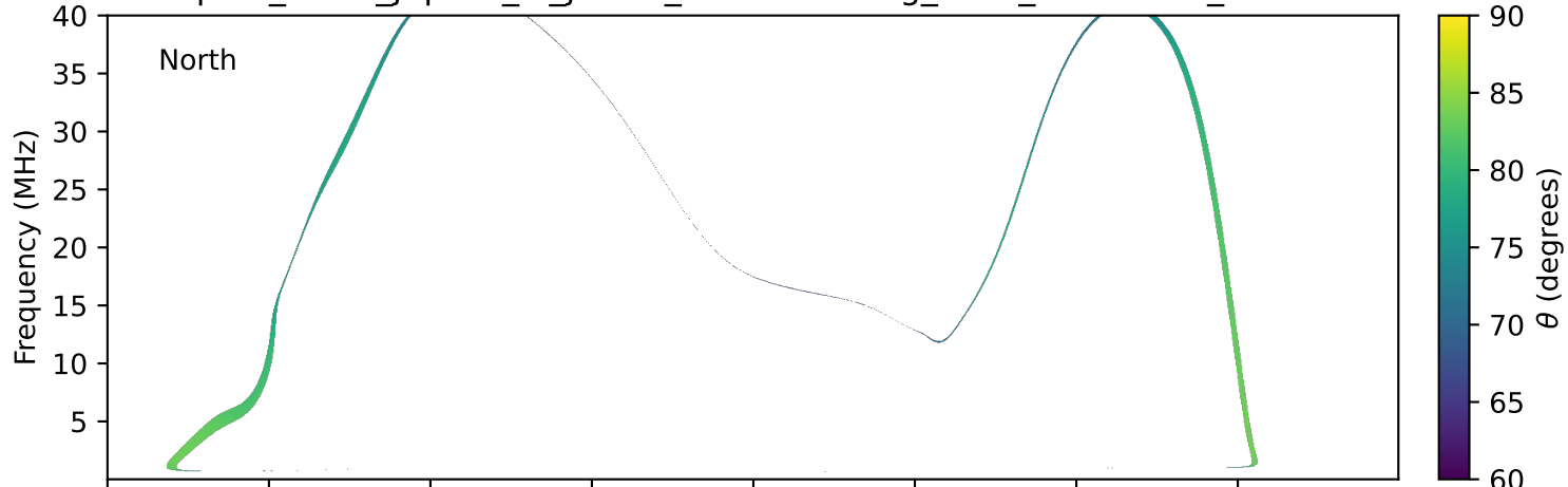
expres_earth_jupiter_io_jrm09_lossc-wid1deg_3kev_19930926_v11.cdf
