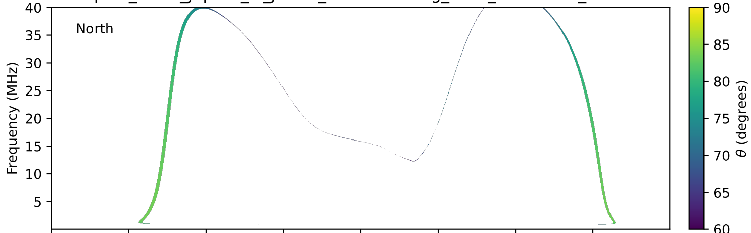
expres_earth_jupiter_io_jrm09_lossc-wid1deg_3kev_19930919_v11.cdf
