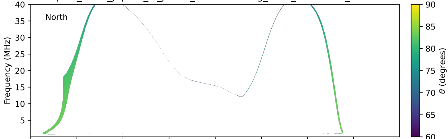
expres_earth_jupiter_io_jrm09_lossc-wid1deg_3kev_19930912_v11.cdf
