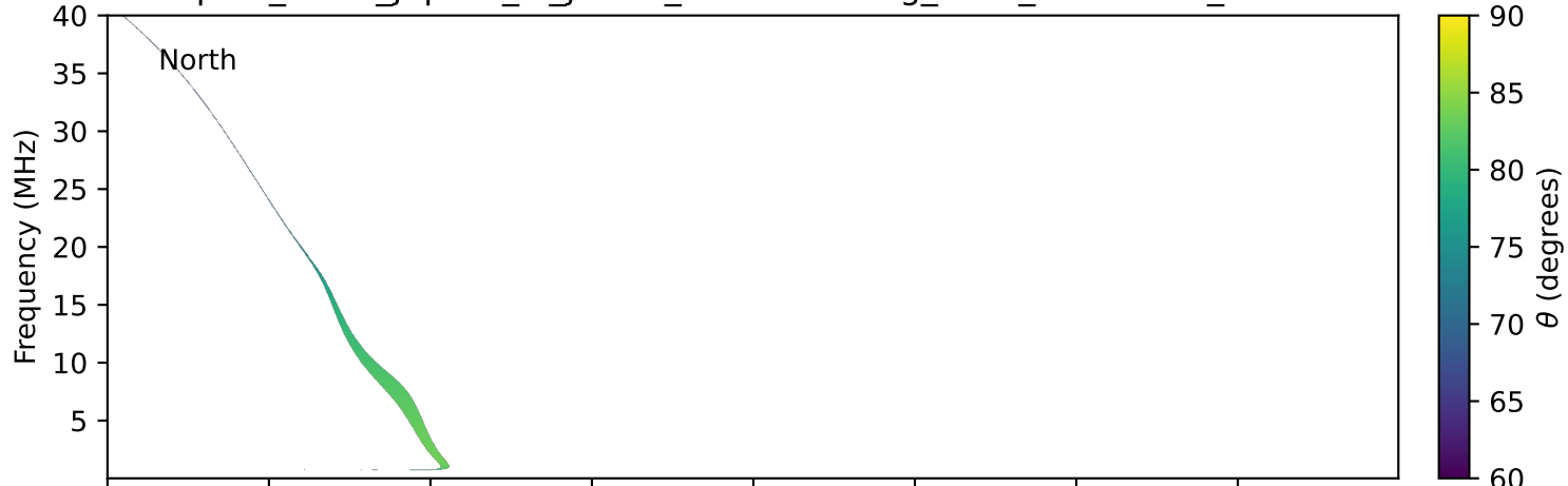
expres_earth_jupiter_io_jrm09_lossc-wid1deg_3kev_19930909_v11.cdf
