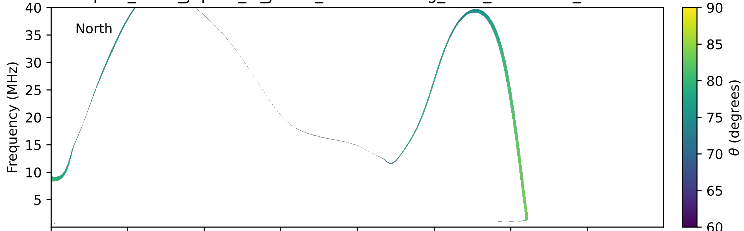
expres_earth_jupiter_io_jrm09_lossc-wid1deg_3kev_19930905_v11.cdf
