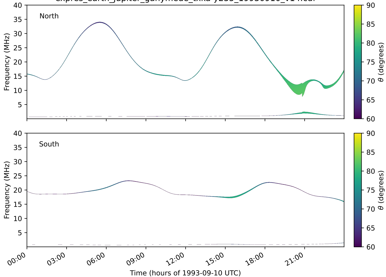
expres_earth_jupiter_ganymede_txka-y235_19930910_v14.cdf
