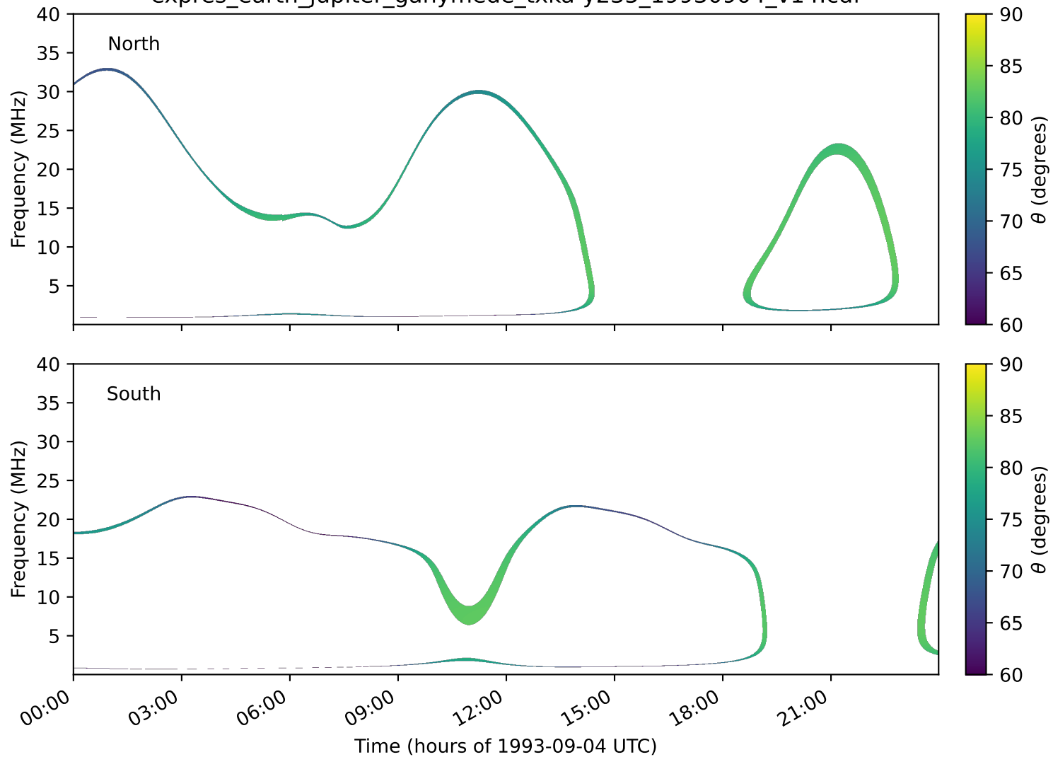
expres_earth_jupiter_ganymede_txka-y235_19930904_v14.cdf
