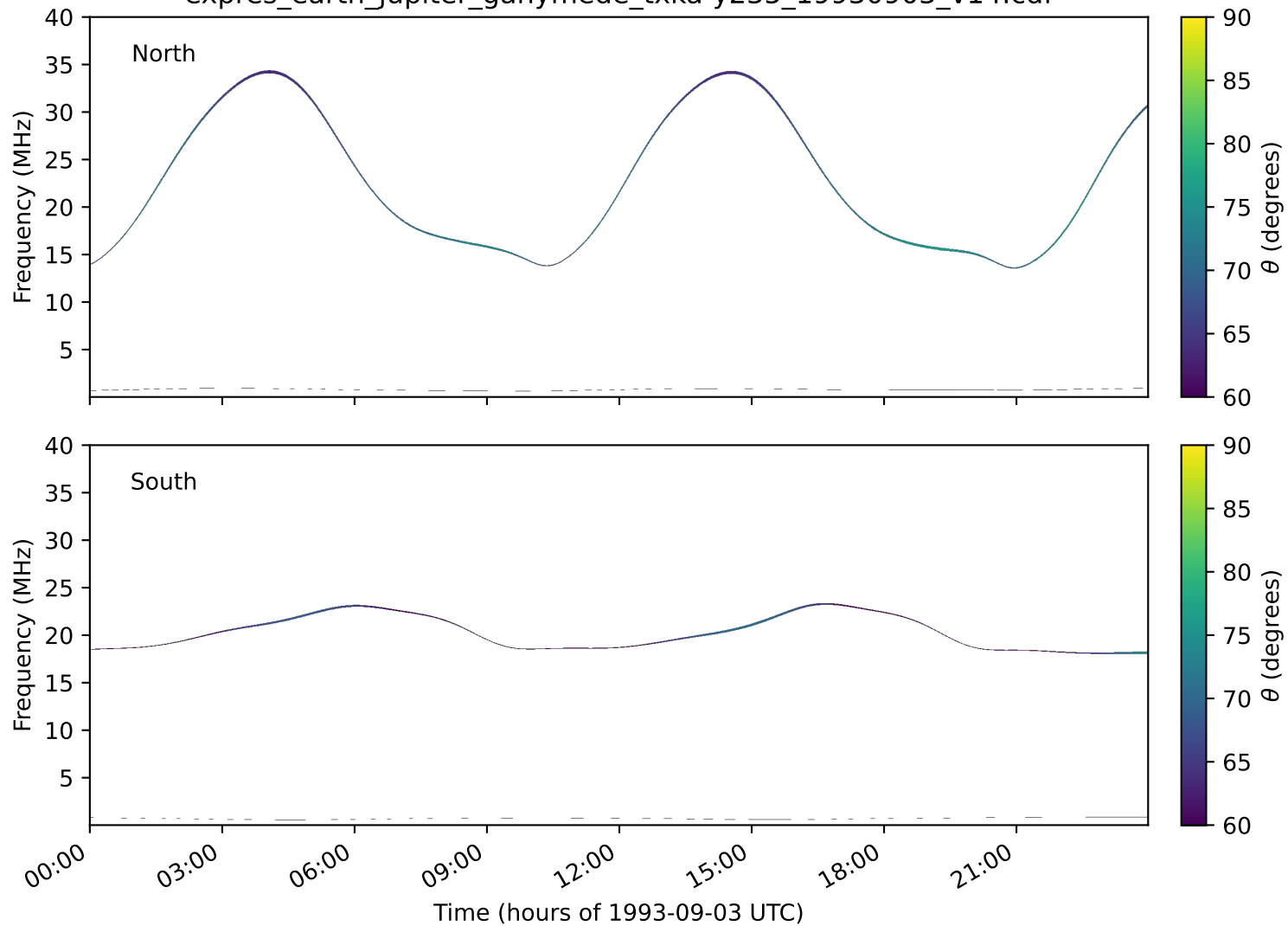
expres_earth_jupiter_ganymede_txka-y235_19930903_v14.cdf
