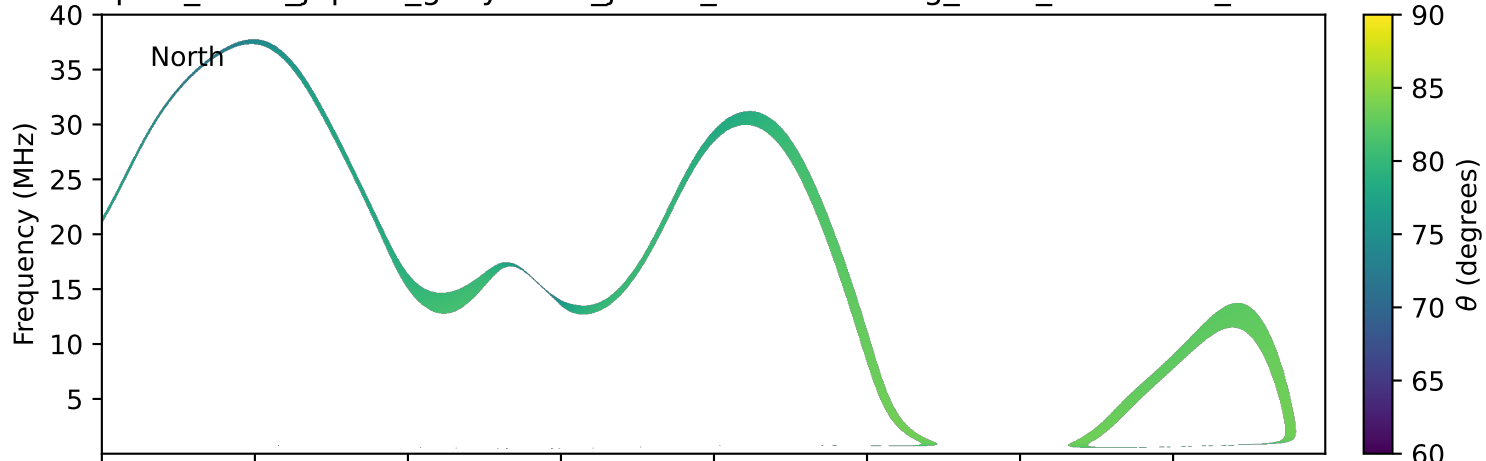
expres_earth_jupiter_ganymede_jrm33_lossc-wid1deg_3kev_19930918_v11.cdf
