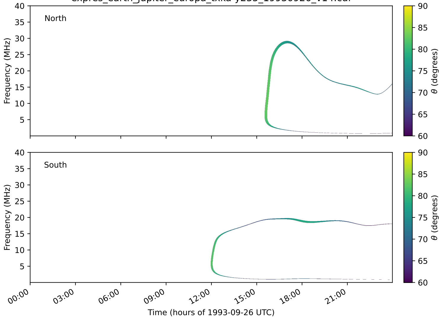
expres_earth_jupiter_europa_txka-y235_19930926_v14.cdf
