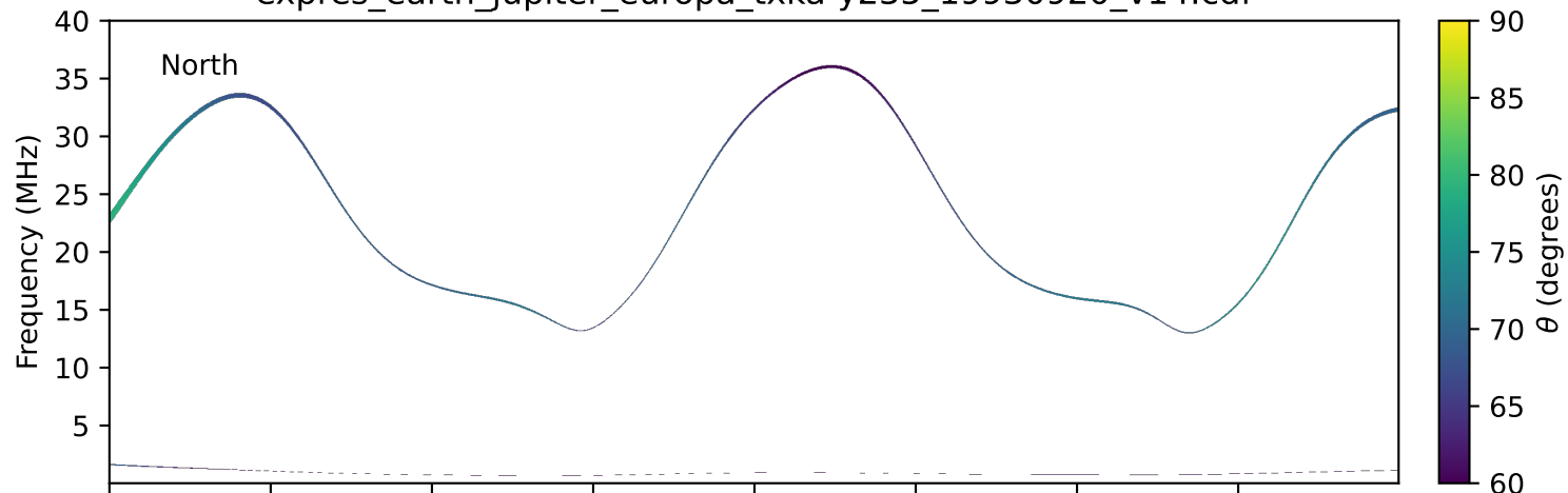
expres_earth_jupiter_europa_txka-y235_19930920_v14.cdf
