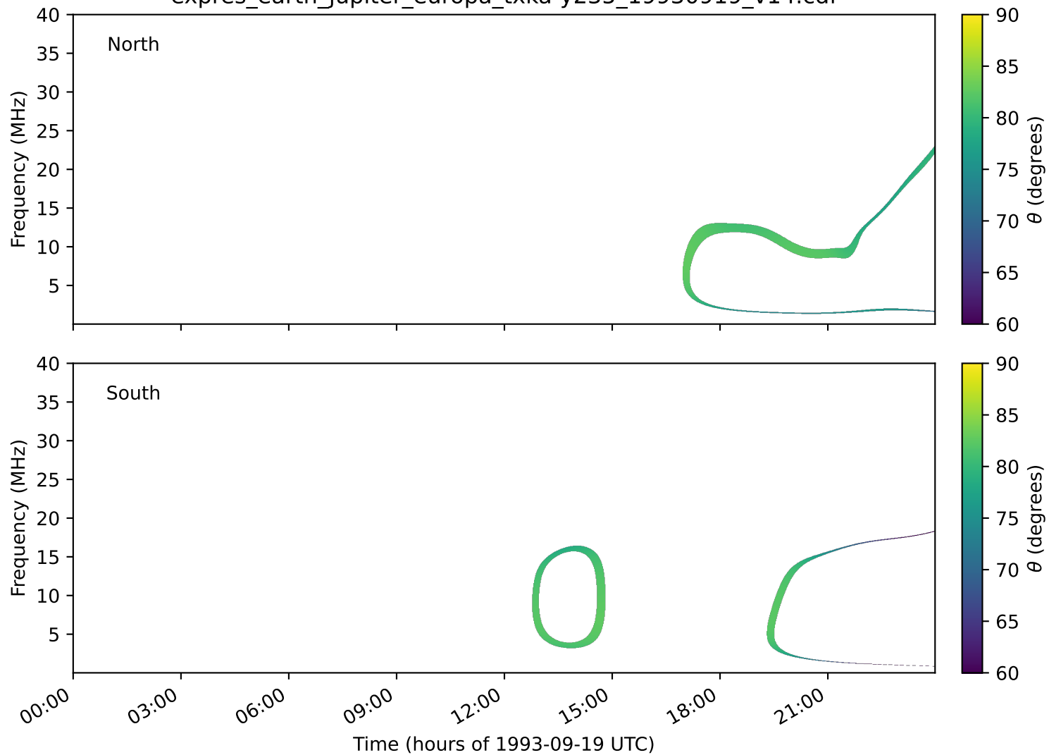
expres_earth_jupiter_europa_txka-y235_19930919_v14.cdf
