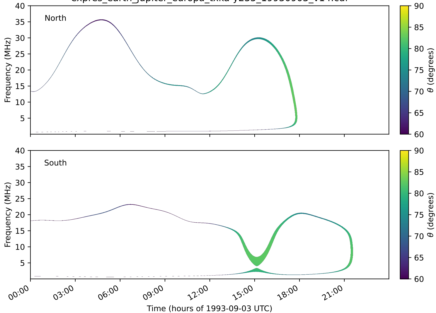
expres_earth_jupiter_europa_txka-y235_19930903_v14.cdf
