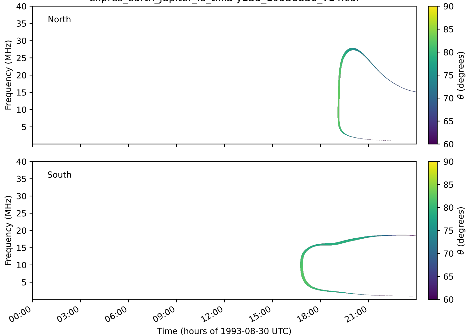
expres_earth_jupiter_io_txka-y235_19930830_v14.cdf
