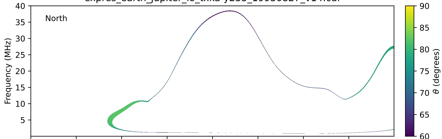
expres_earth_jupiter_io_txka-y235_19930827_v14.cdf
