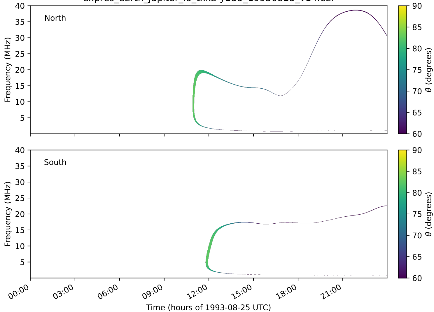
expres_earth_jupiter_io_txka-y235_19930825_v14.cdf
