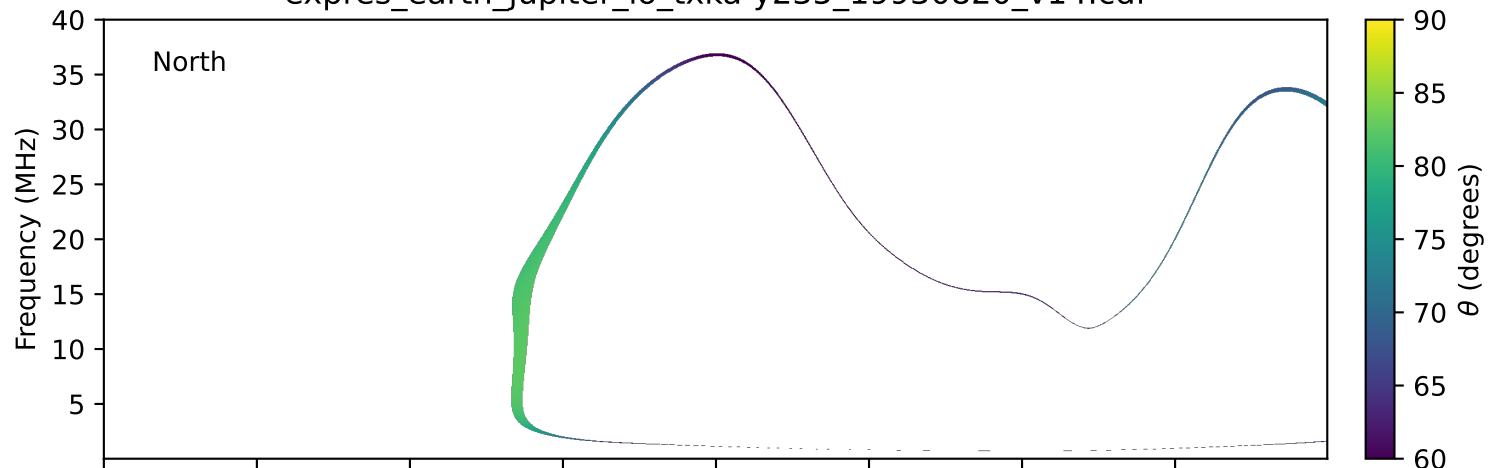
expres_earth_jupiter_io_txka-y235_19930820_v14.cdf
