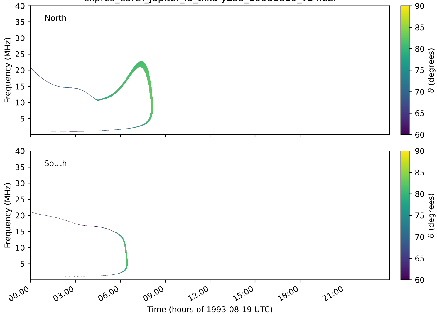
expres_earth_jupiter_io_txka-y235_19930819_v14.cdf
