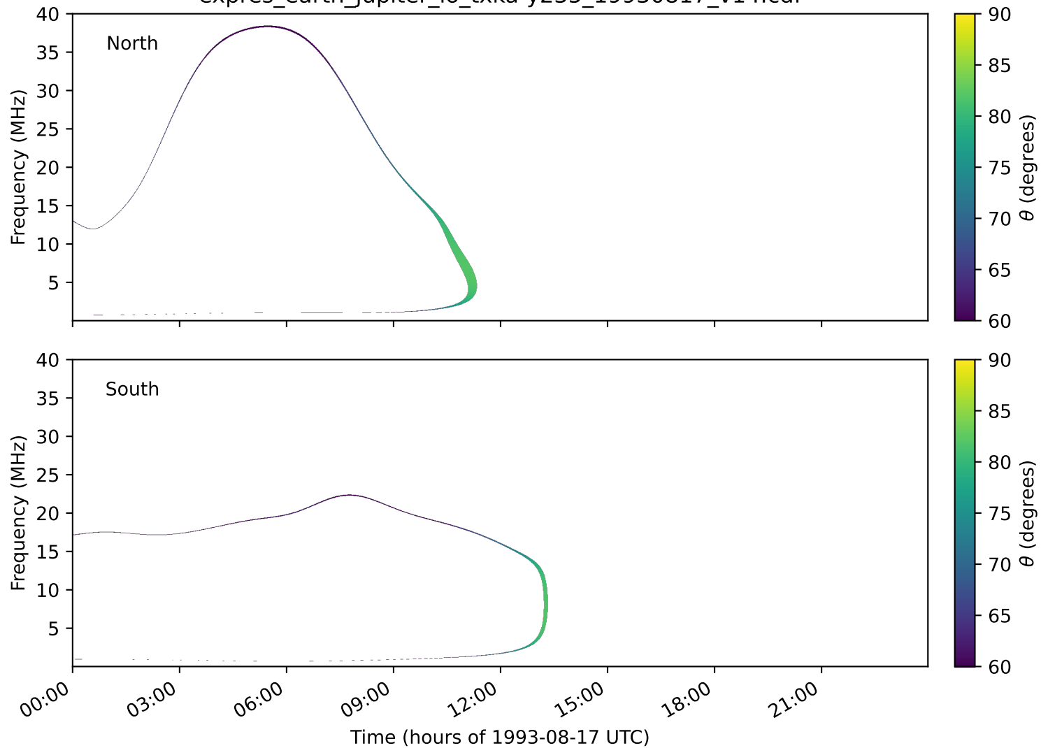
expres_earth_jupiter_io_txka-y235_19930817_v14.cdf
