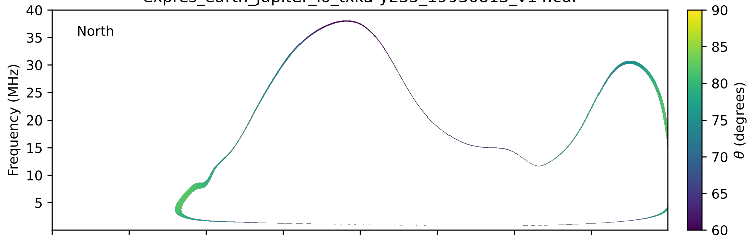
expres_earth_jupiter_io_txka-y235_19930813_v14.cdf
