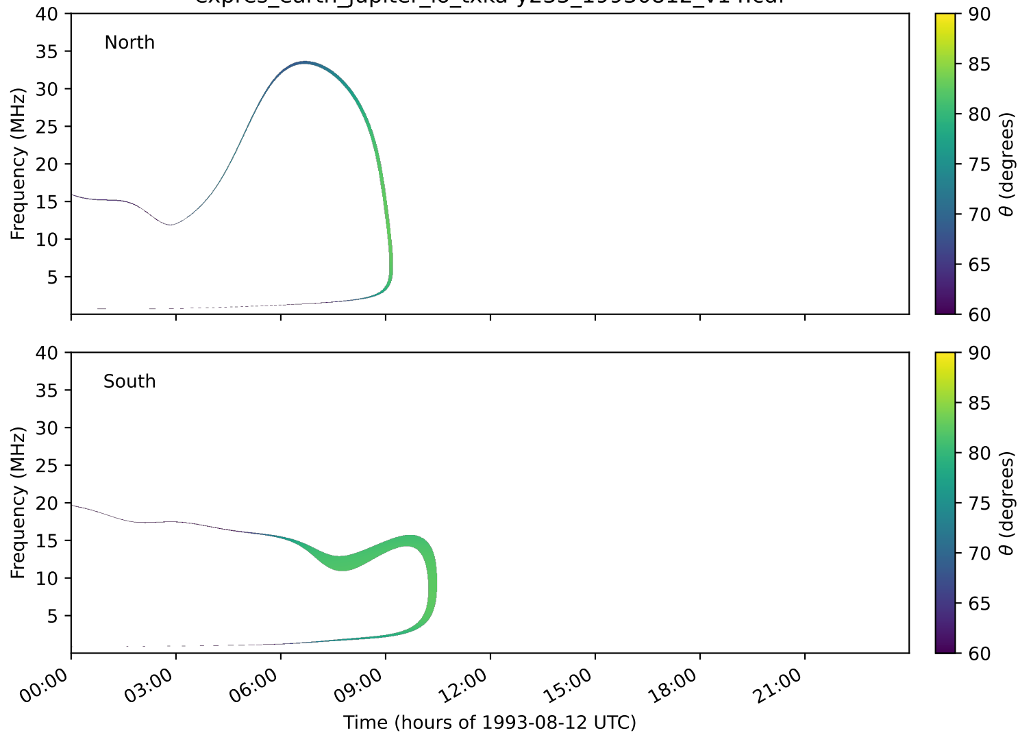
expres_earth_jupiter_io_txka-y235_19930812_v14.cdf
