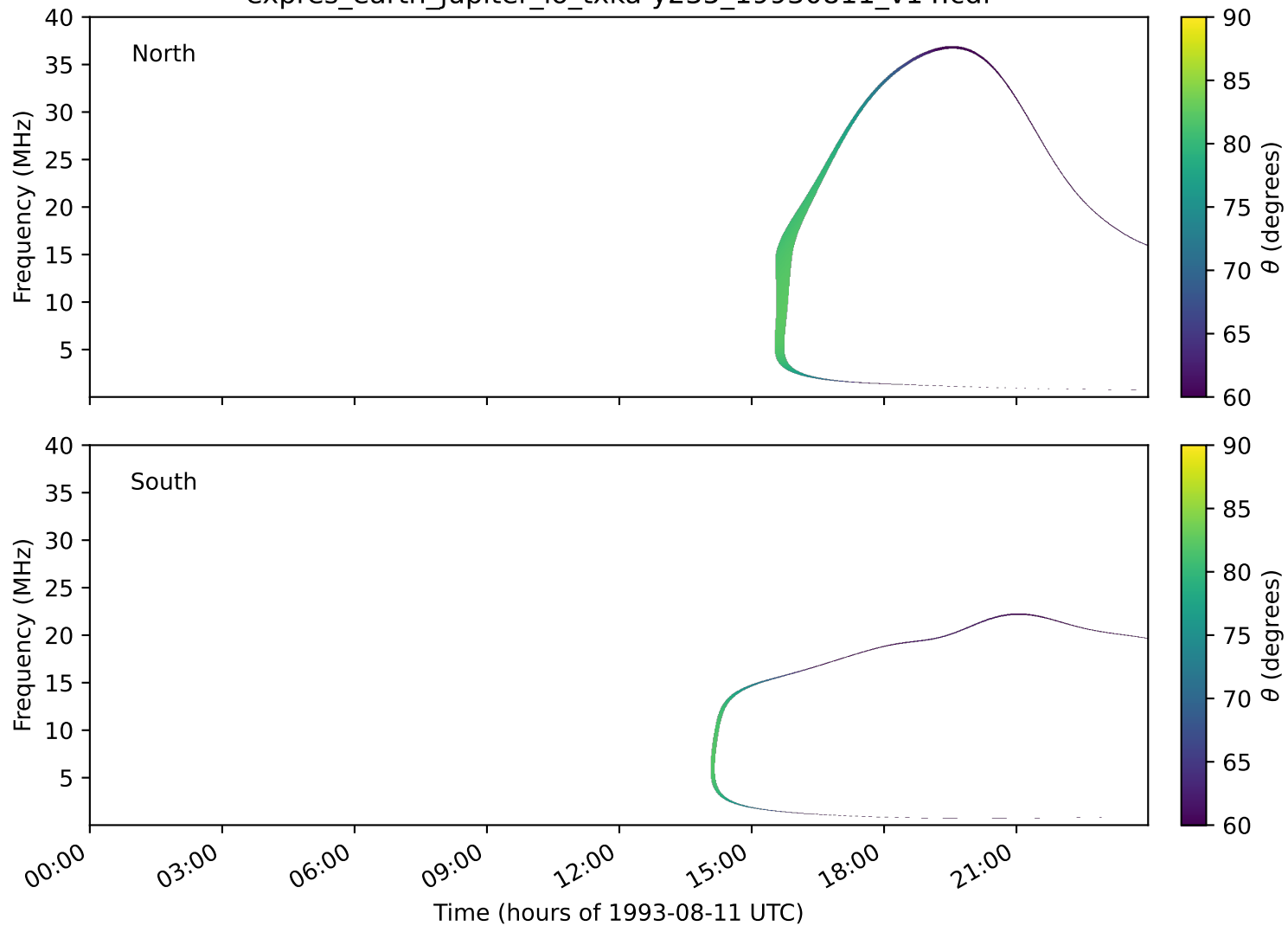
expres_earth_jupiter_io_txka-y235_19930811_v14.cdf
