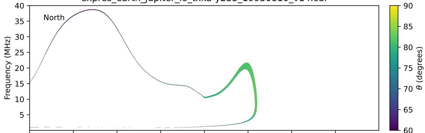
expres_earth_jupiter_io_txka-y235_19930810_v14.cdf
