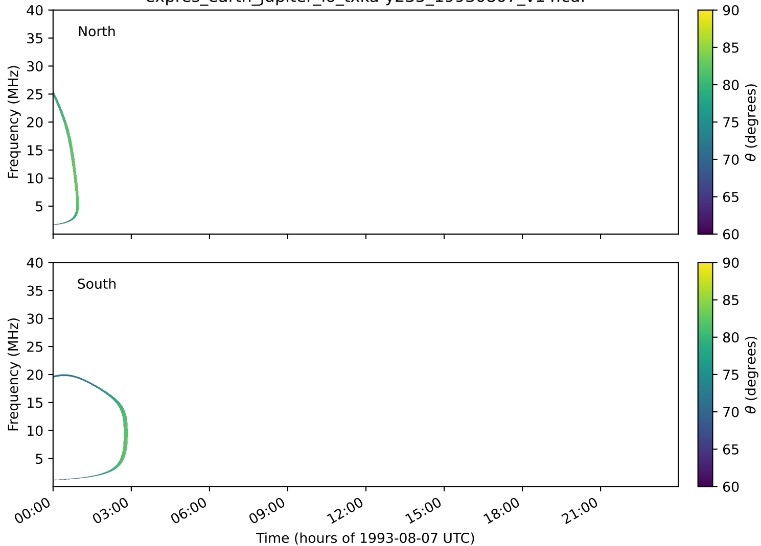
expres_earth_jupiter_io_txka-y235_19930807_v14.cdf
