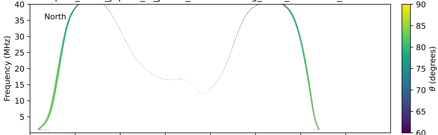
expres_earth_jupiter_io_jrm33_lossc-wid1deg_3kev_19930829_v11.cdf
