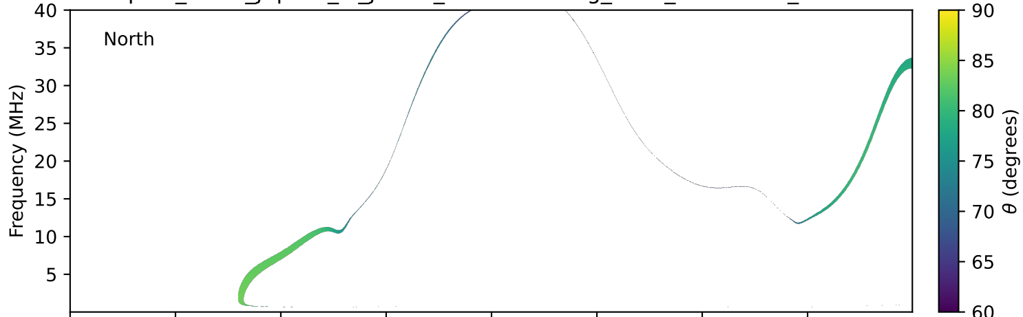
expres_earth_jupiter_io_jrm33_lossc-wid1deg_3kev_19930827_v11.cdf
