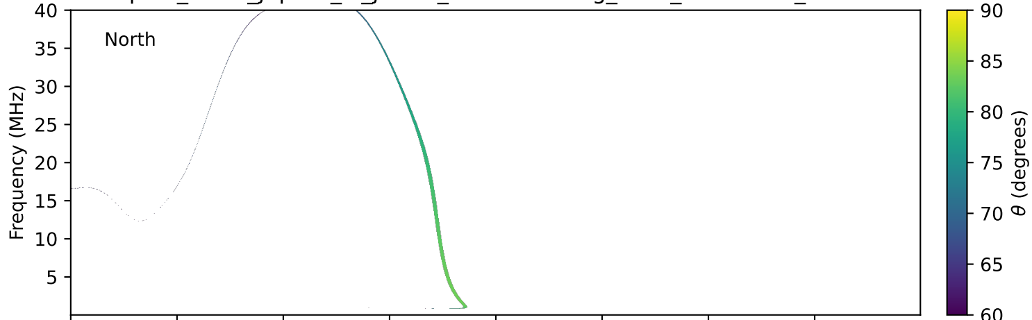
expres_earth_jupiter_io_jrm33_lossc-wid1deg_3kev_19930824_v11.cdf
