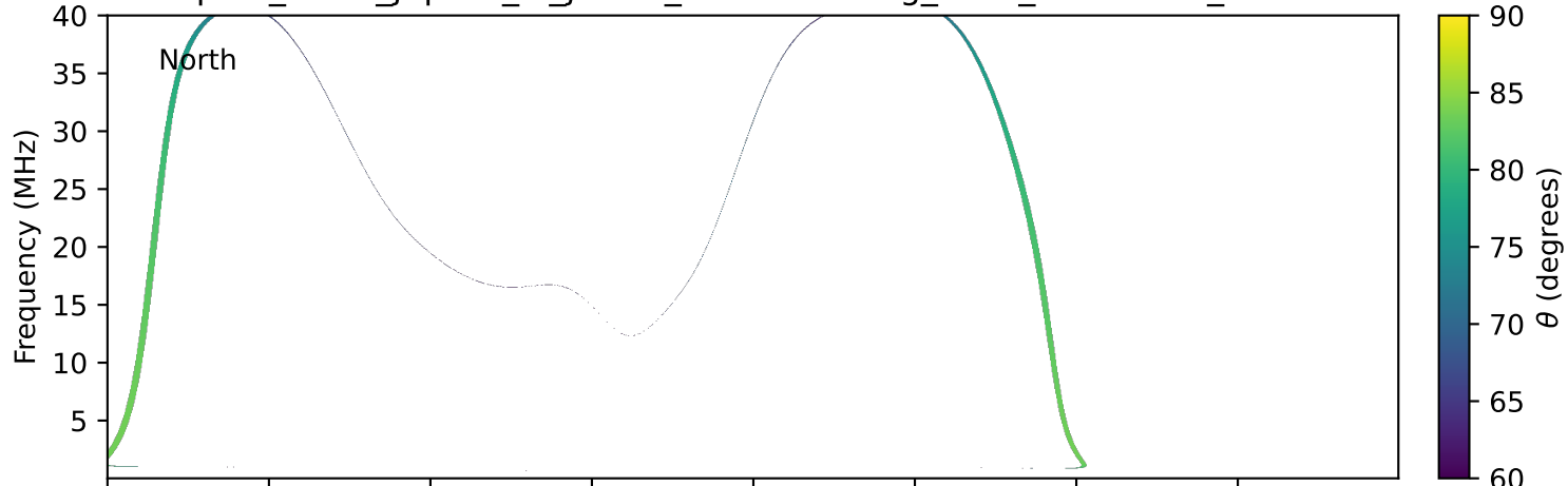
expres_earth_jupiter_io_jrm33_lossc-wid1deg_3kev_19930815_v11.cdf
