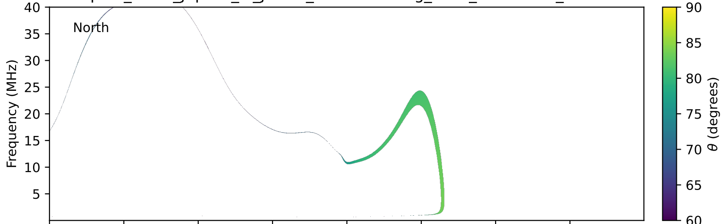
expres_earth_jupiter_io_jrm33_lossc-wid1deg_3kev_19930810_v11.cdf
